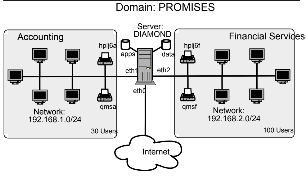
Figure 3.1 Abmas Network Topology — 130 Users
